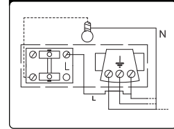
Connection Diagram
